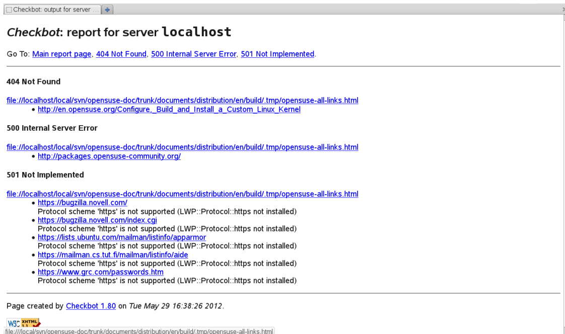
FIGURE 3.1: EXAMPLE OUTPUT OF daps linkcheck
